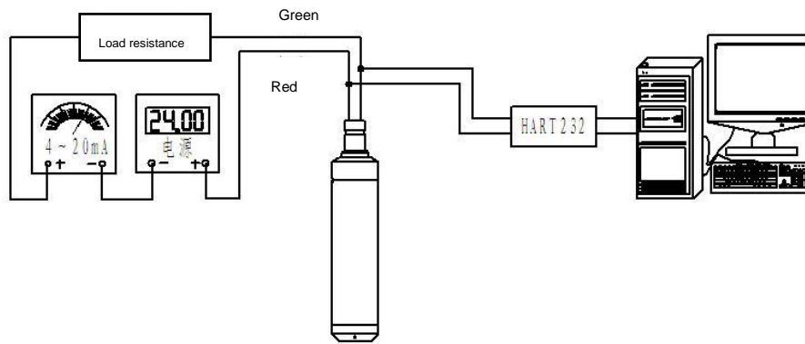
Pressure transmitter configuration system with HART protocol
